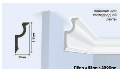
115mm x 55mm x 2000mm
