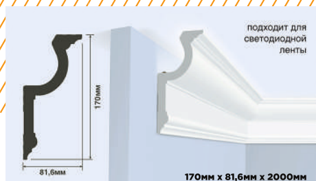
170mm x 81.6mm x 2000mm
